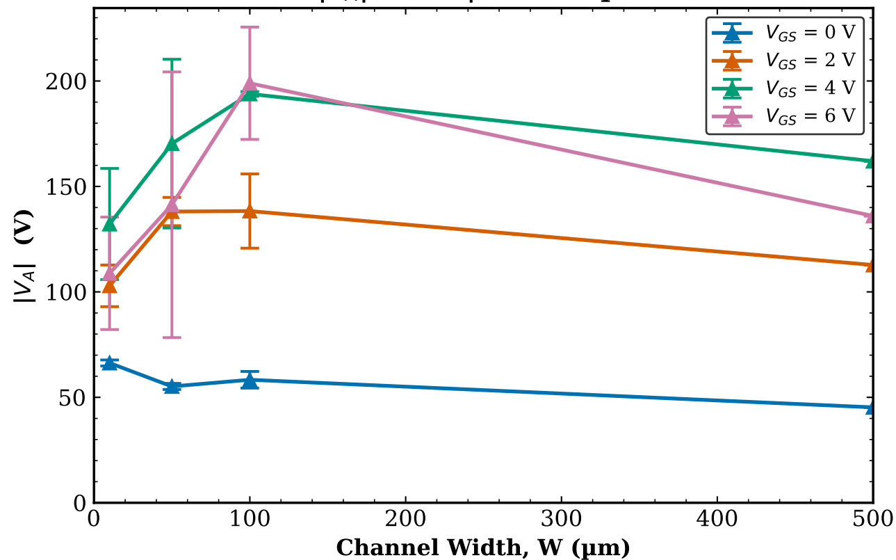
TFT1 Combined (Tr. 1 & 2) |V_A| vs W | L = 40\text{ }\mu\text{m}
